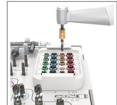
6. Handpiece lifted with the drill stop now attached to the drill.
